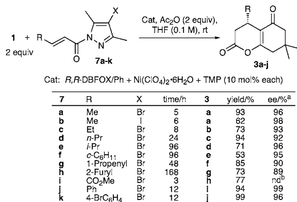
Scheme 3. Nickel(II)-Catalyzed Enantioselective Synthesis of a Variety of Enol Lactones
