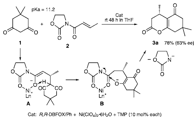
Scheme 1. Nickel(II)-Catalyzed Enantioselective Enol Lactone Formation
