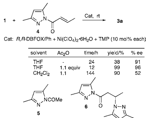
Scheme 2. Solvent and Additive Effect in the Enol Lactone Formation
