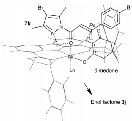
Figure 1. Suggested transition model to rationalize the stereoselectivity observed in the R,R -DBFOX/Ph complex catalyzed reaction.
